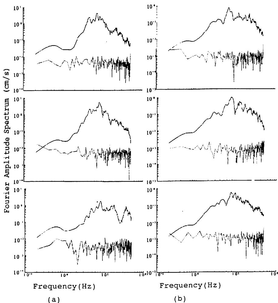
Fig. 8 Fourier amplitude spectra of Event 03, M_L=4.0 , Oct. 4, 1994; (a) surface; (b) downhole; From the top to the bottom is the component of R, T, and V respectively; Solid line is the spectra of signal and dash line is the spectra of noise.
