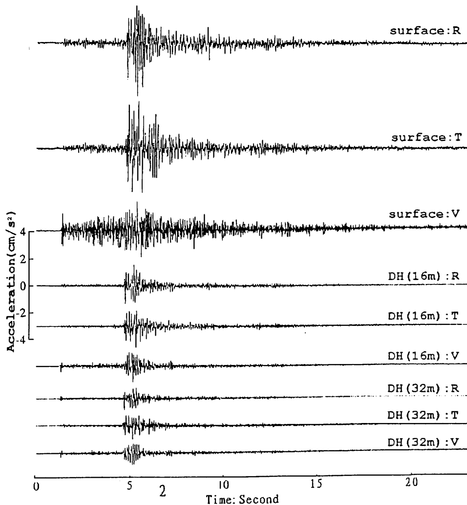
Fig. 7 Accelerograms generated by the Event 17, M_L=3.0 , June 27, 1995; Parameters of the earthquake are: origin time: 06/27/1995, 22:46:18.6 BT; focal depth: 13 km; epicenter location: 39^\circ 44'N , 118^\circ 27'E ; epicenter distance: 24.7 km; backazimuth 280^\circ .
