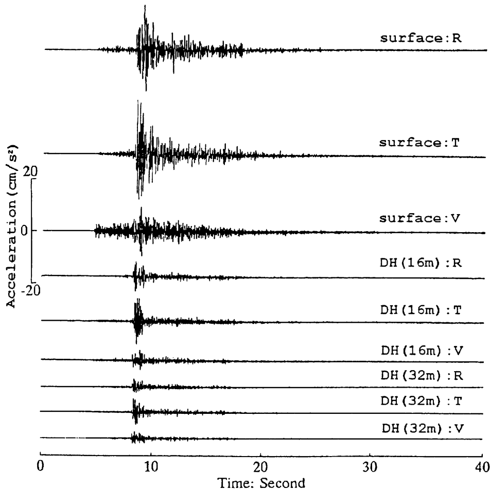
Fig. 6 Accelerograms generated by the Event 03, M_L=4.0 , October 4, 1994; Parameters of the earthquake are: origin time: 10/04/1994, 15:54:17.2 BT; focal depth: 11 km; epicenter location: 39° 44'N, 118° 26'E; epicenter distance: 26 km; backazimuth 279°.
