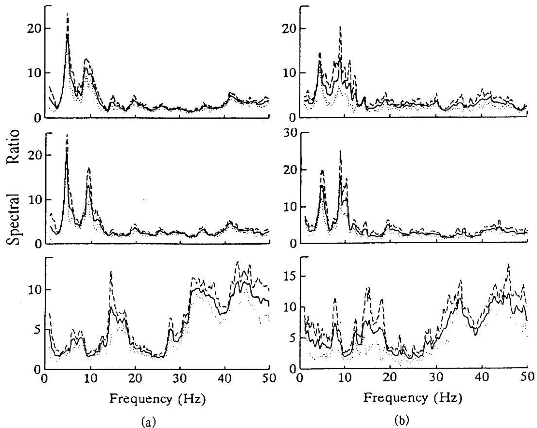
Fig. 13 The mean spectral ratio of 0m/32m: (a) Group one including Event 03, 16, 17, 22, 23, 25; (b) Group two including Event 13, 14, 18, 20,21, 24. From the top to the bottom is the component R, T and V respectively
