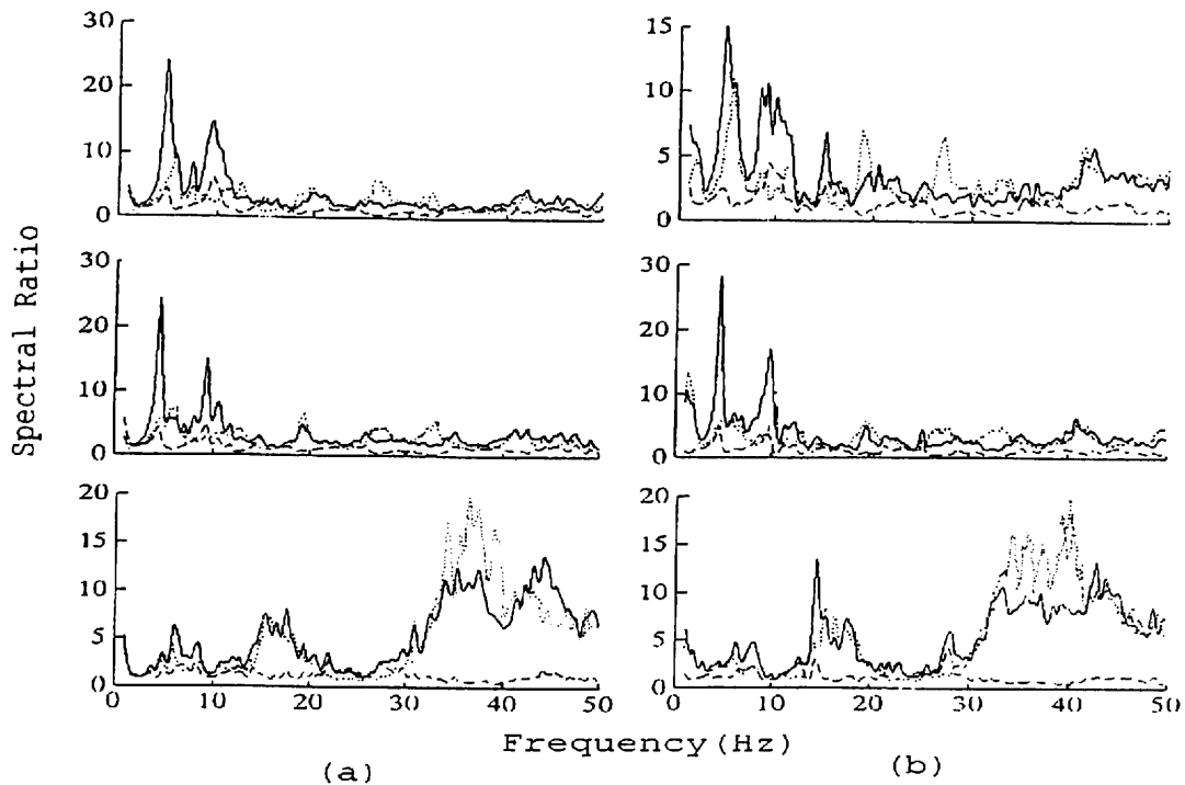
Fig 9 Spectral ratio: (a) Event 03, M_L=4.0 , Oct. 4, 1994; (b) Event 17, M_L=3.0 , Jun. 27, 1995; From the top to the bottom is the component of R, T, and V respectively; Solid line is 0m/32m, dash line is 16m/32m, and dot line is 0m/16m.
