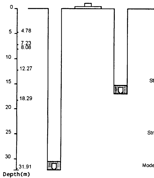
Fig. 3 Location of the sensors
